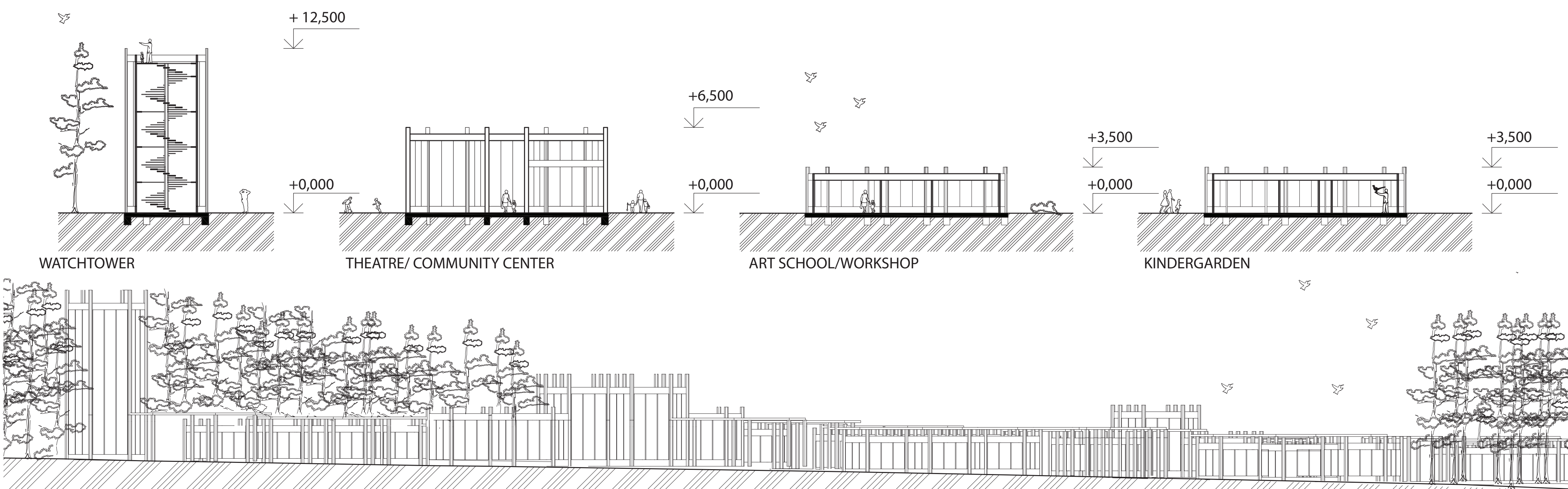
SECTION VIEW OF SELECTED OBJECTS, M 1:200
